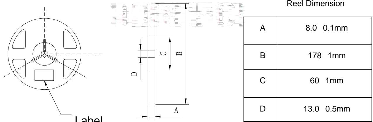
Fig.2-2 Reel Dimension
