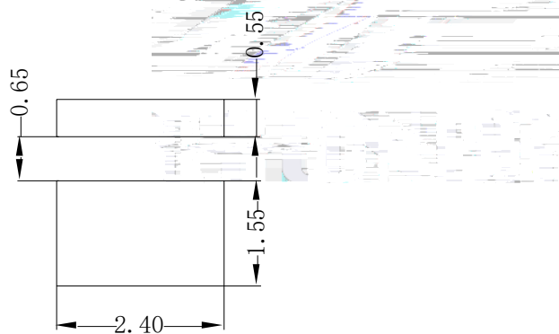
Fig.1-5 Soldering Patterns
