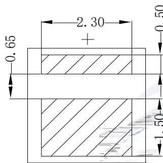
Fig.1-3 Bottom View
