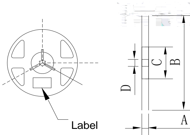
Fig.2-2 Reel Dimension
