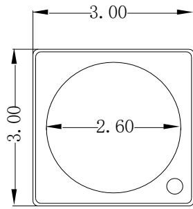
Fig.1-1 Top View
