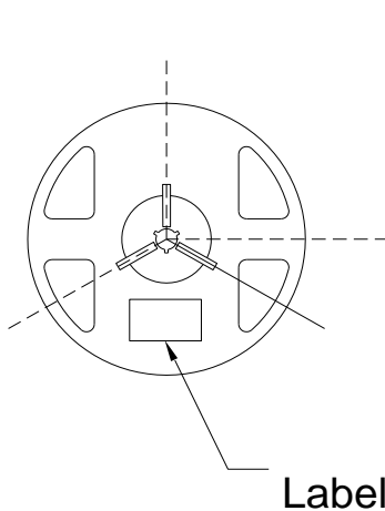
Fig.2-2Reel Dimension 卷盘
