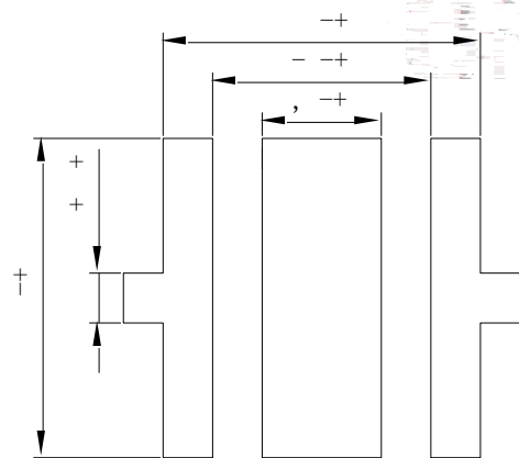
Fig.1-5 Soldering patterns
