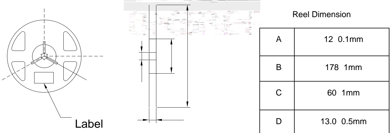
Fig.2-2 Reel Dimension
