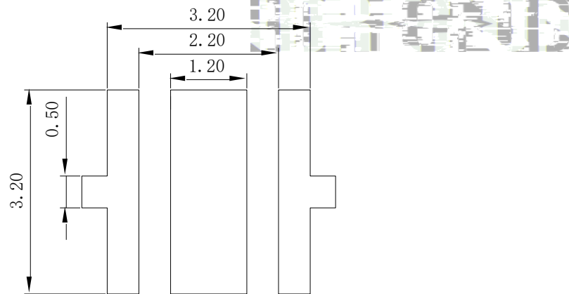
Fig.1-5 Soldering patterns
