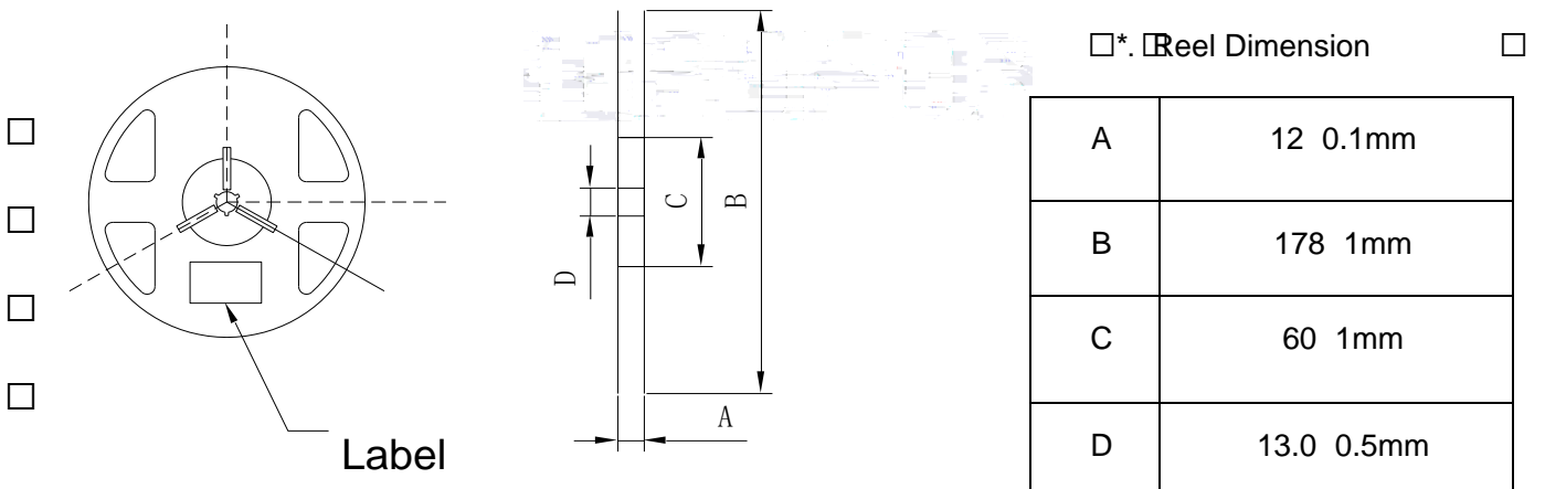
Fig.2-2 Reel Dimension
