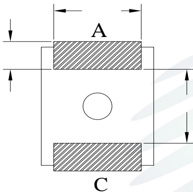
Fig. 1-3 Bottom View
