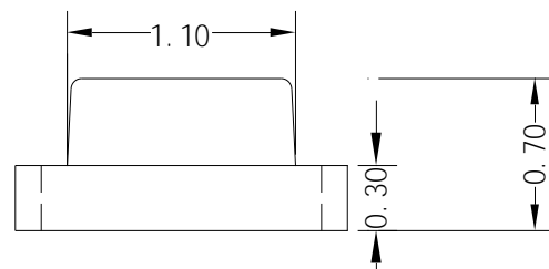
Fig.1-2 Side view
