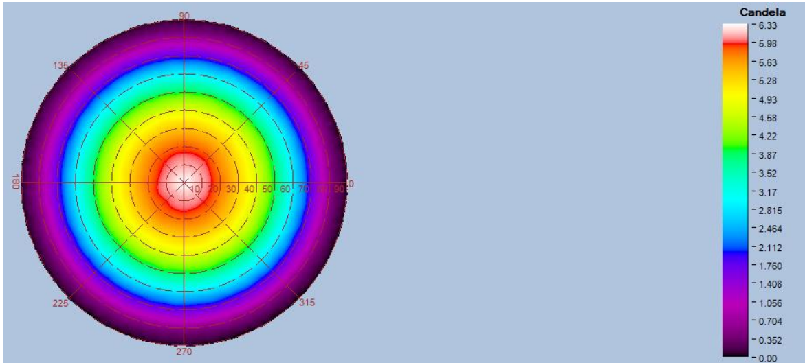
Intensity(traced to infinity) Cross Section Luminous Intensity(Candela)
